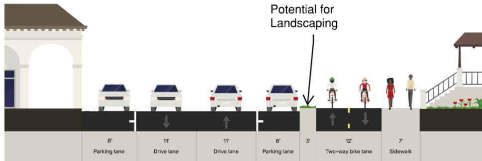
Conceptual Cross section 1 Santa Fe St - Tulare Ave to Cypress Ave
