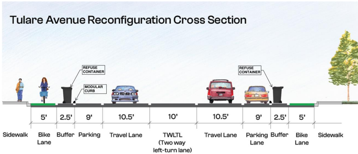
Figure 1 – Tulare Avenue Cross Section
