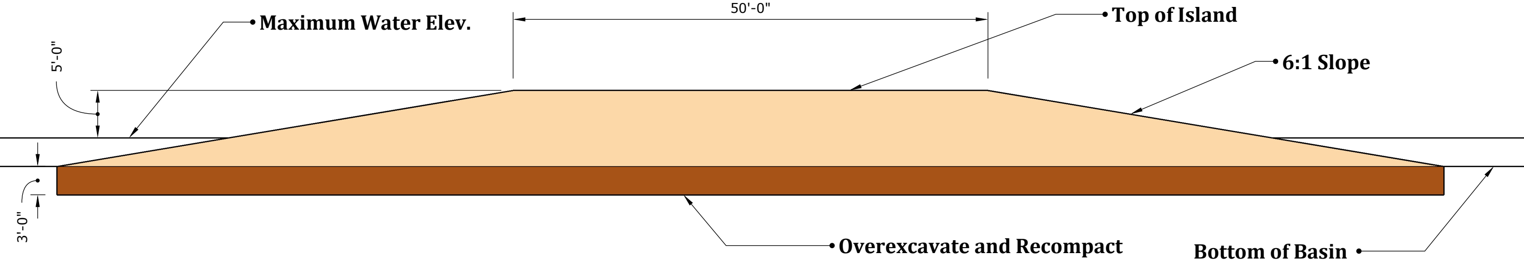
Island Cross Section
