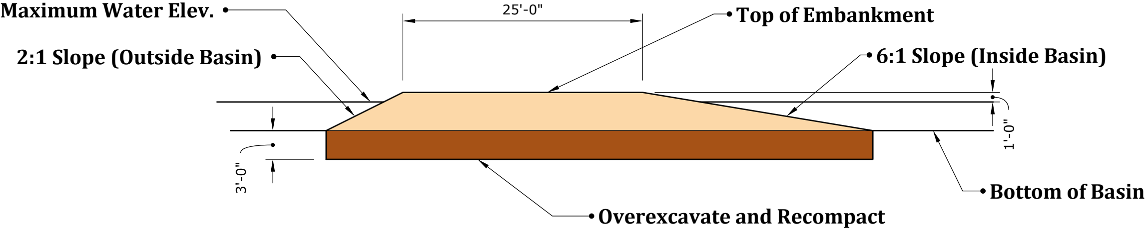
Embankment Cross Section
