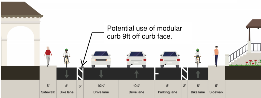
Conceptual Cross section 2 Highland Project - Houston St from Bridge St to Santa Fe St
