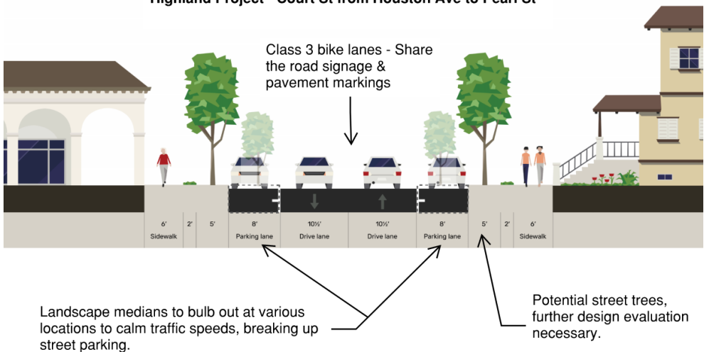
Conceptual Cross section 3 Highland Project - Court St from Houston Ave to Pearl St
