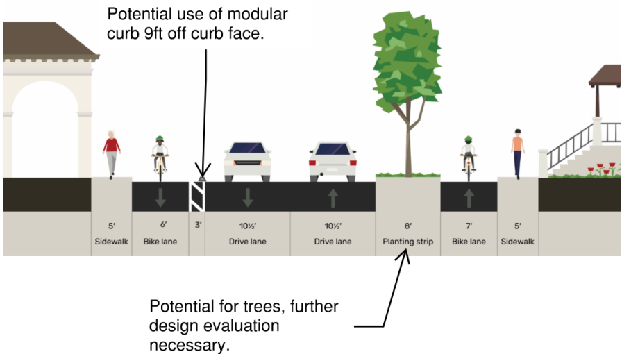
Conceptual Cross section 3 Highland Project - Court St from Houston Ave to Pearl St
