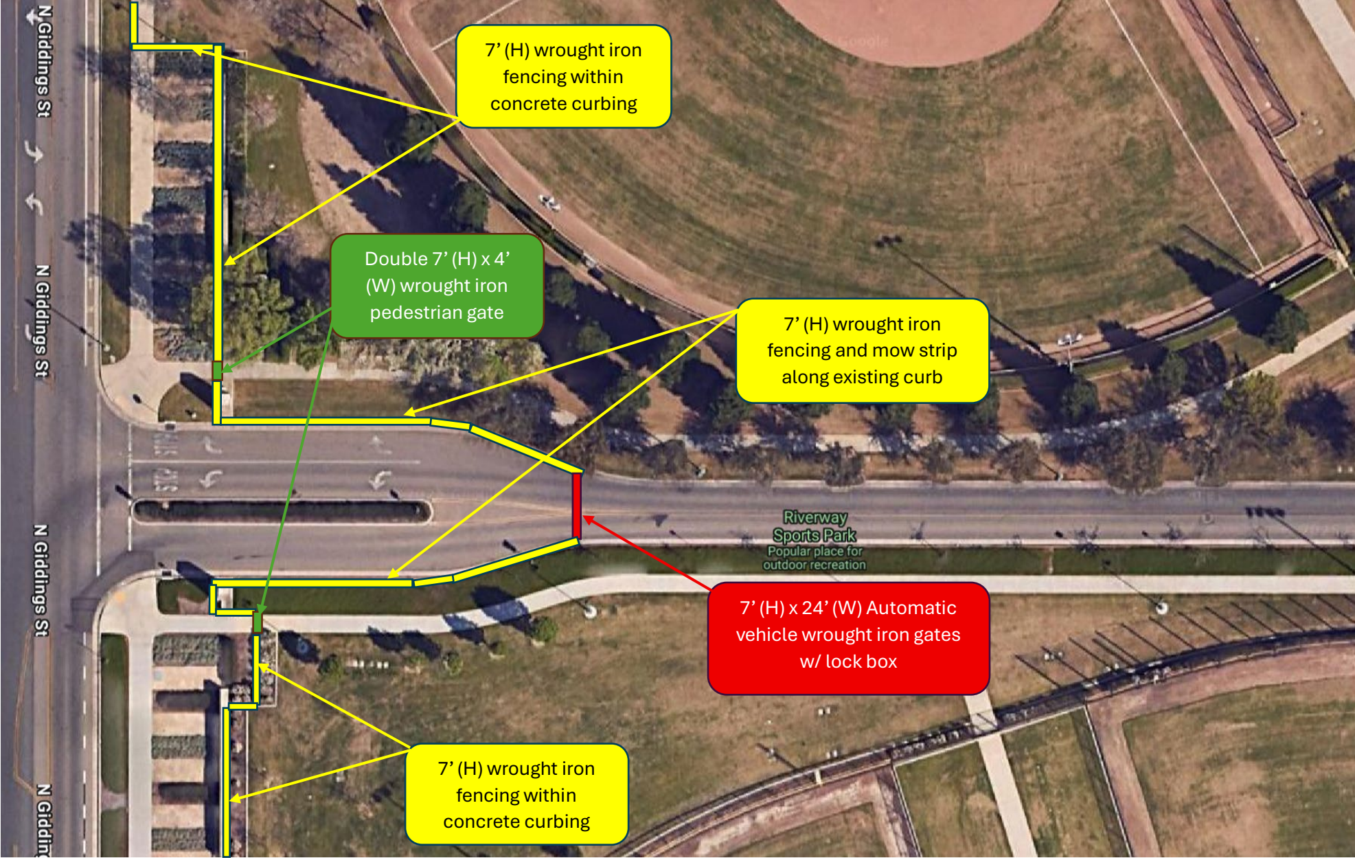
Site Map - Giddings Entrance Exhibit “J”
