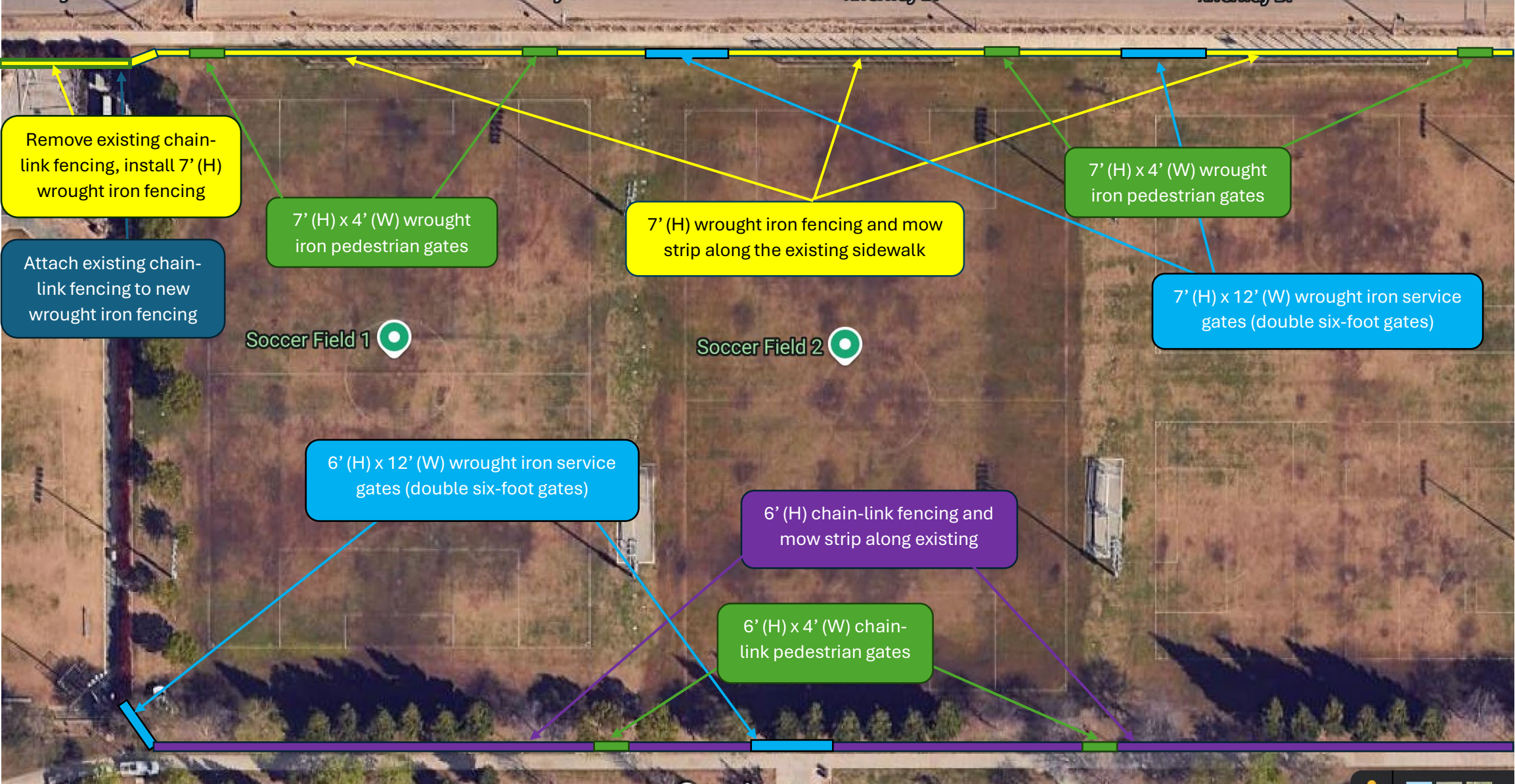
Site Map - North Side Fields 1, 2, & 3 Exhibit "A"
