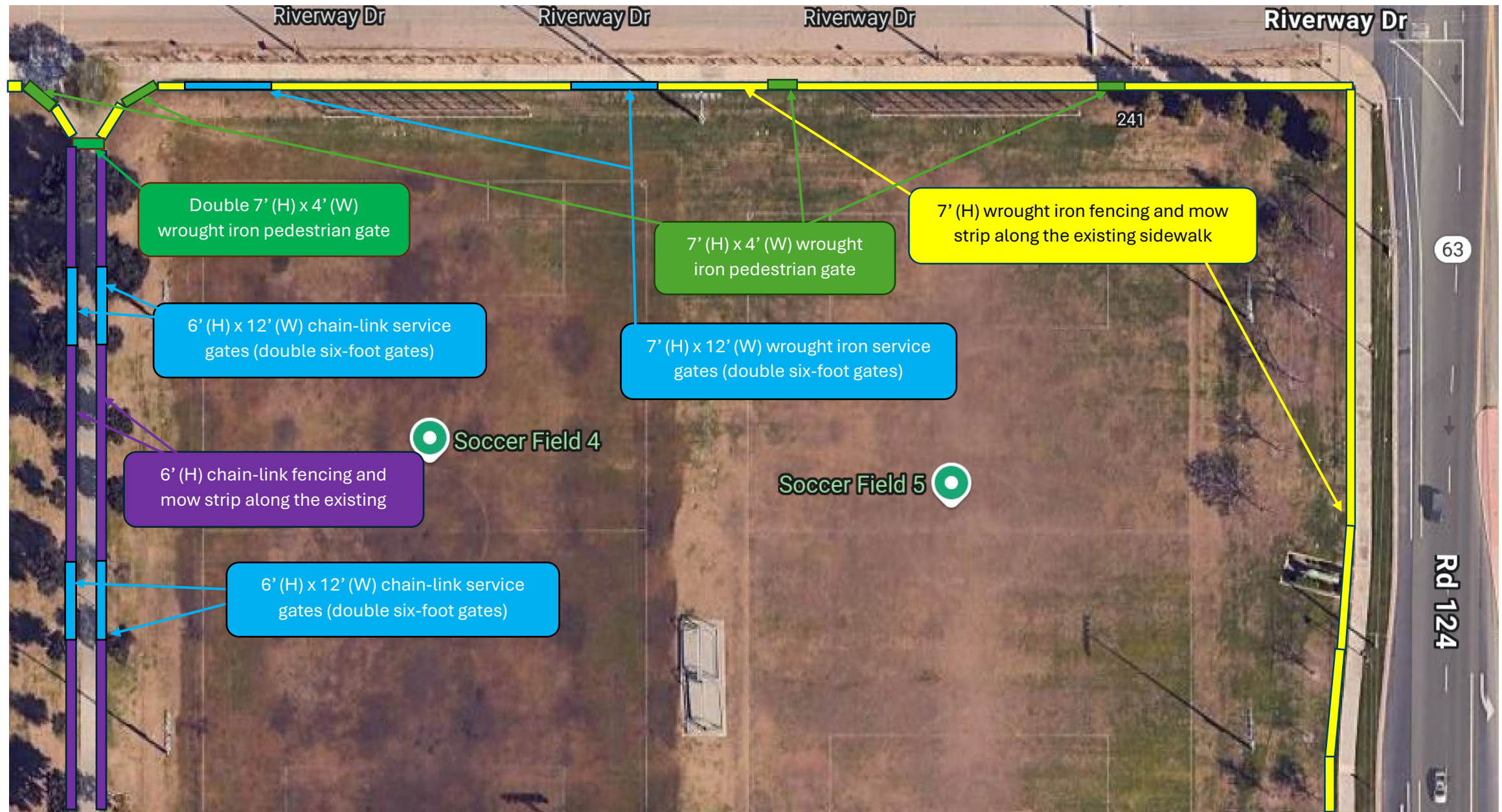
Site Map - North Side Fields 4 & 5 Exhibit "B"
