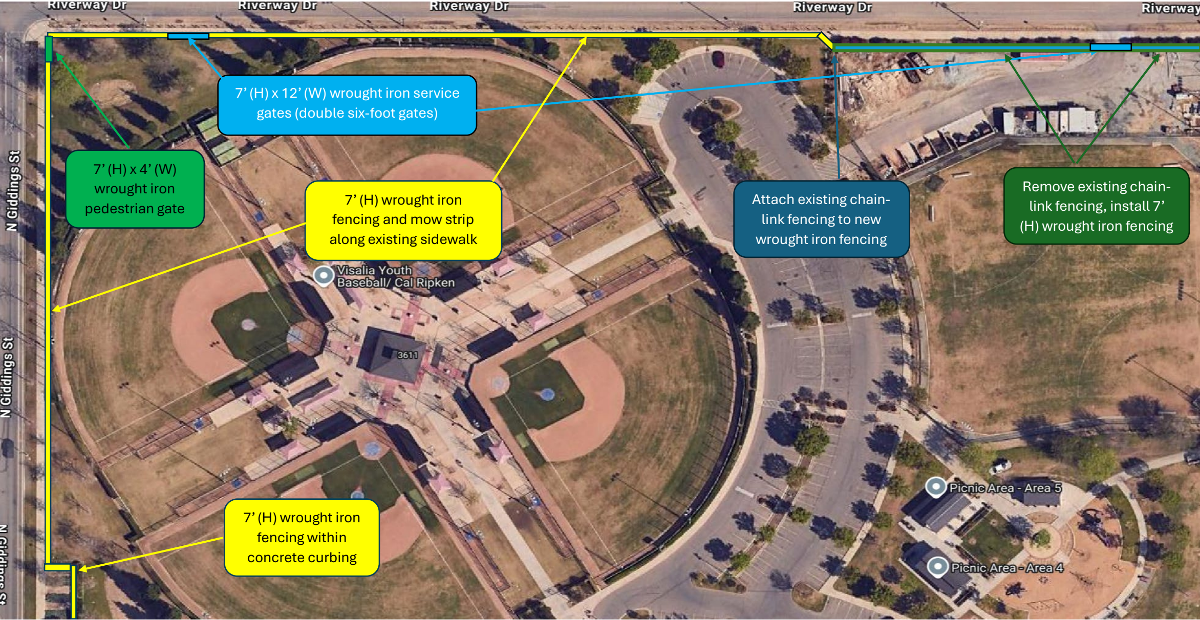
Site Map - CR Shannon Fields Exhibit "K"
